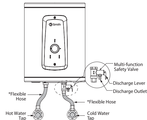
Figure 12 Installation Diagram
